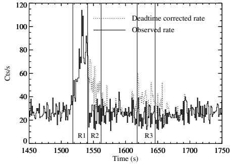
Figure 1. The observed (solid histogram) and the reconstructed (dashed histogram) light curve of ME events in 100–500 keV band. The gaps are treated as dead-time. The vertical solid lines separate R1, R2, R3 regions (see text).
