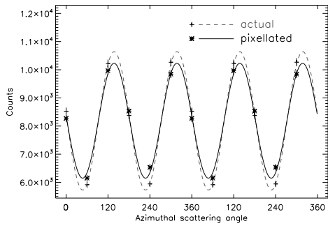
Figure 3. Simulated azimuthal scattering angle distribution of 100% polarized photons at 200 keV originating at the GRB position. Solid fit is for pixellated, and dashed fit is for interaction positions within the detectors
